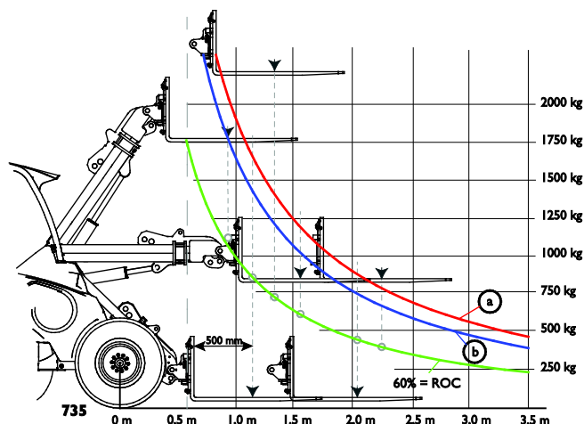
Lastdiagram 735
